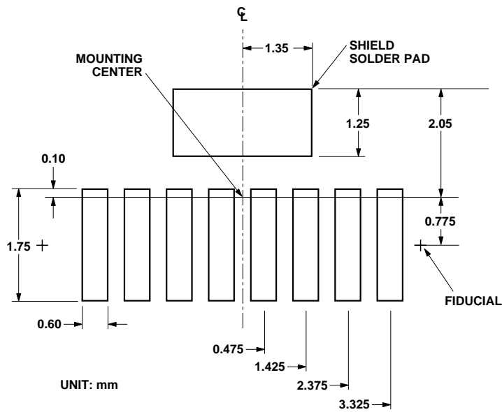
Figure 13. Land pattern.
